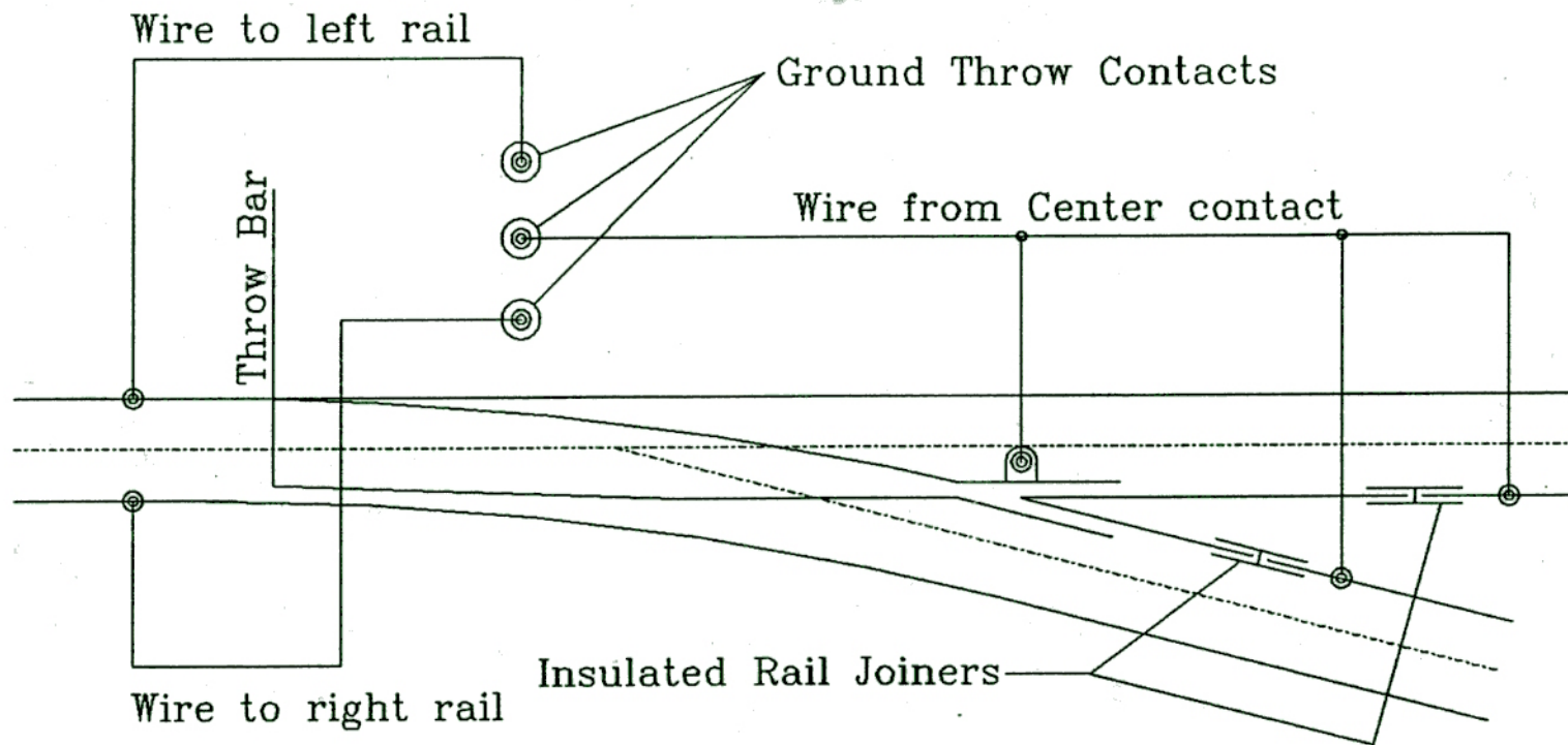
Turnout Power Distribution For sidings with Atlas@ Turnouts
